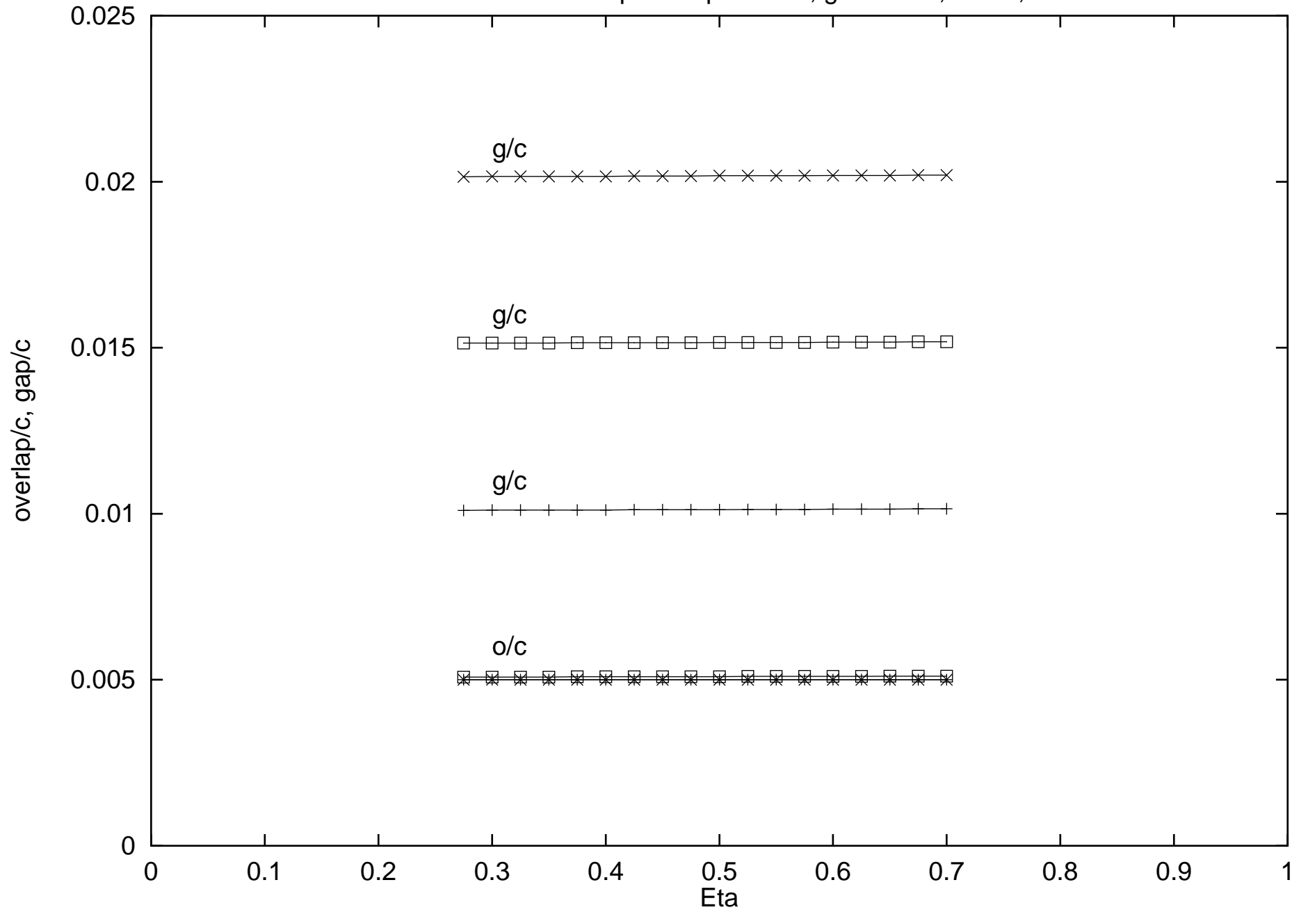
Position Check for Partspan Flap - df=20 , g/c=0.010, 0.015, 0.020
