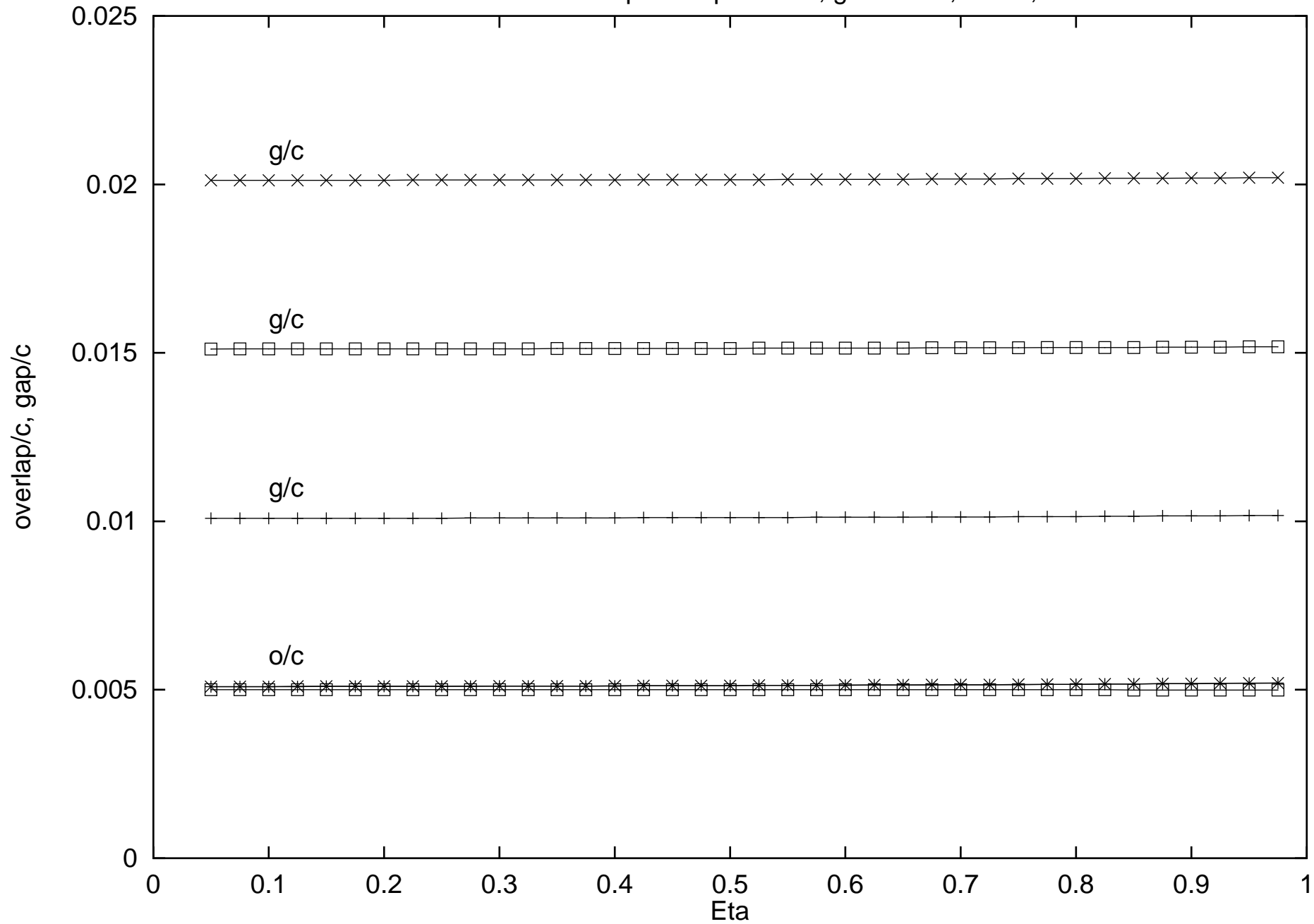
Position Check for Fullspan Flap - df=25 , g/c=0.010, 0.015, 0.020
