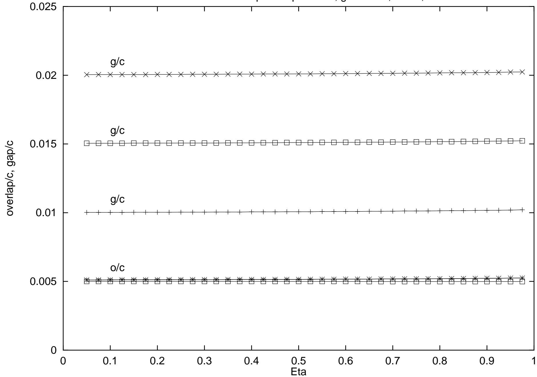
Position Check for Fullspan Flap - df=30 , g/c=0.010, 0.015, 0.020
