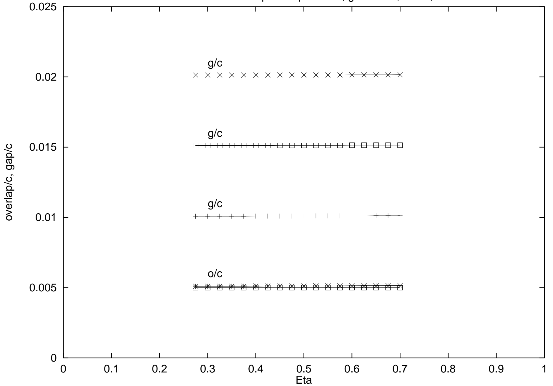
Position Check for Partspan Flap - df=25 , g/c=0.010, 0.015, 0.020
