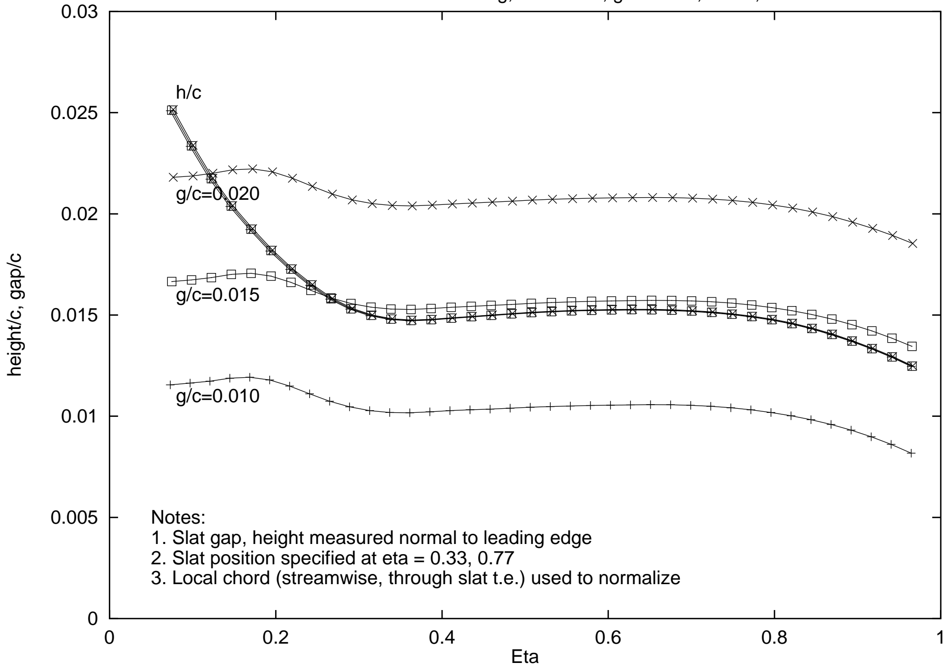
Slat Position Check - ds=30 deg, h/c=0.015 , g/c=0.010, 0.015, 0.020
