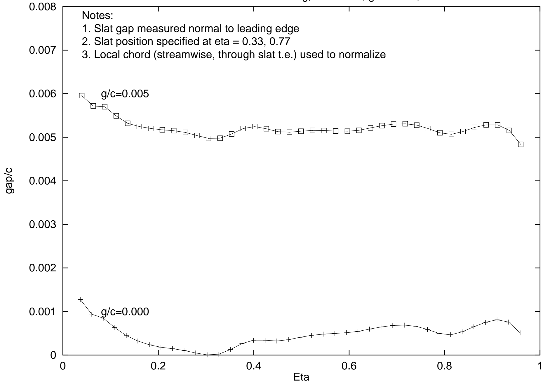
Slat Position Check - ds=20 deg, h/c=0.045 , g/c=0.000, 0.005
